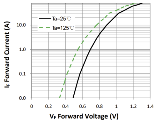
Figure 1. Forward Characteristic(typ.)
