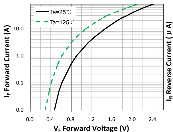
Figure 1. Forward Characteristic(typ.)
