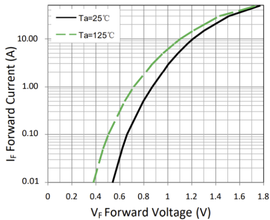
Figure 1. Forward Characteristic(typ.)
