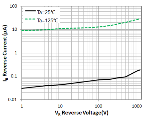
Figure 2. Reverse Characteristic(typ.)
