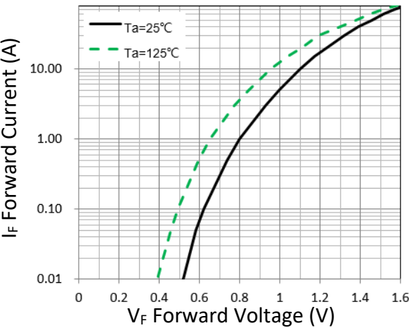
Figure 1. Forward Characteristic(typ.)
