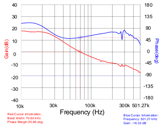
Bode Plot
