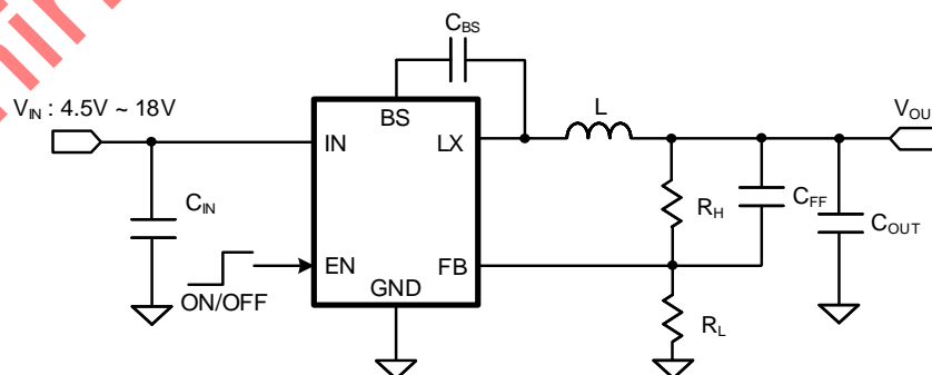
Figure1. Schematic Diagram
