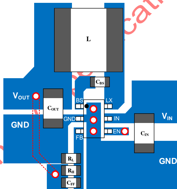
Figure3. Suggested PCB Layout
