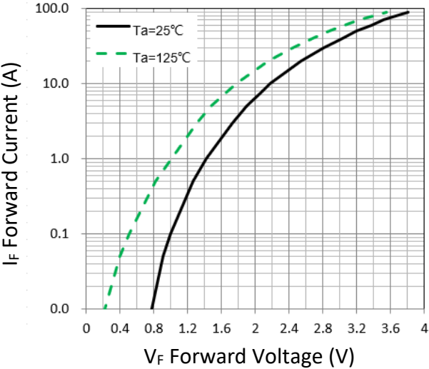
Figure 1. Forward Characteristic(typ.)
