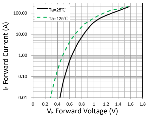
Figure 1. Forward Characteristic(typ.)
