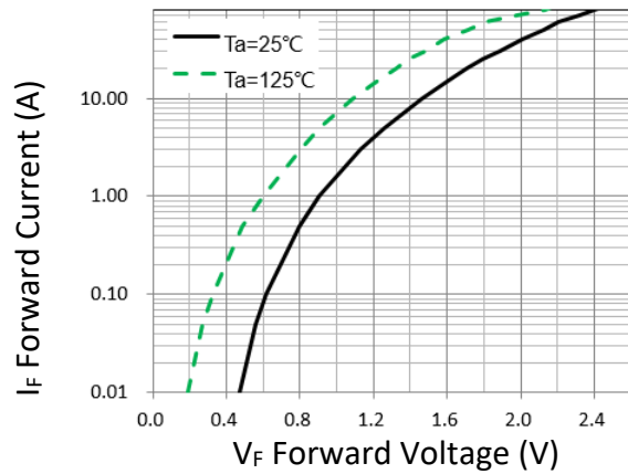
Figure 1. Forward Characteristic(typ.)
