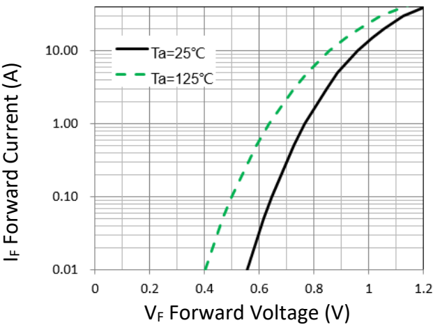
Figure 1. Forward Characteristic(typ.)
