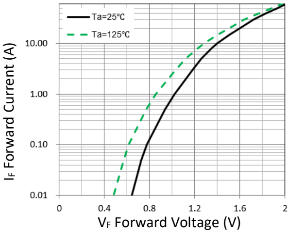
Figure 1. Forward Characteristic(typ.)
