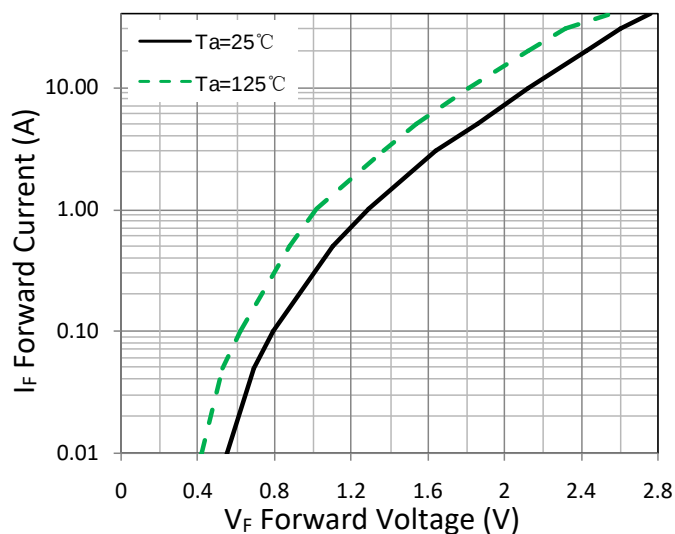
Figure 1. Forward Characteristic(typ.)
