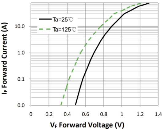
Figure 1. Forward Characteristic(typ.)
