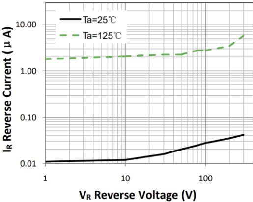
Figure 2. Reverse Characteristic (typ.)
