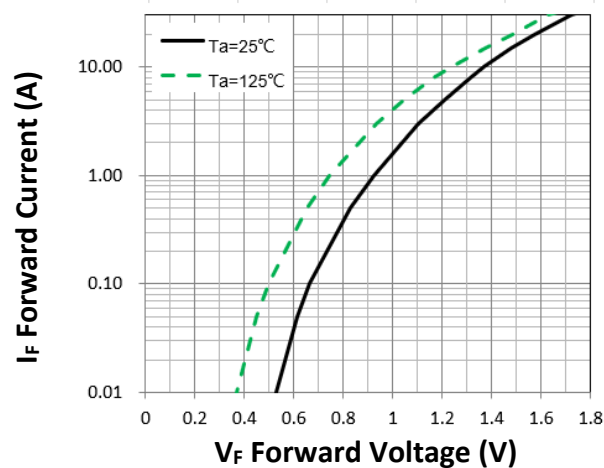
Figure 1. Forward Characteristic(typ.)
