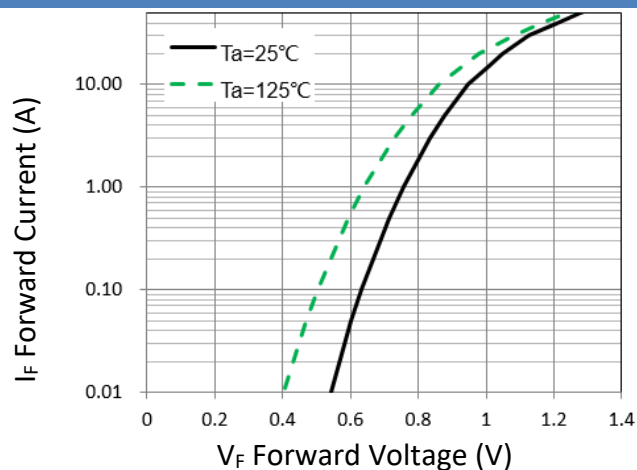
Figure 1. Forward Characteristic(typ.)
