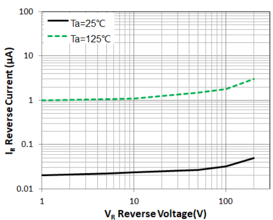
Figure 2. Reverse Characteristic(typ.)
