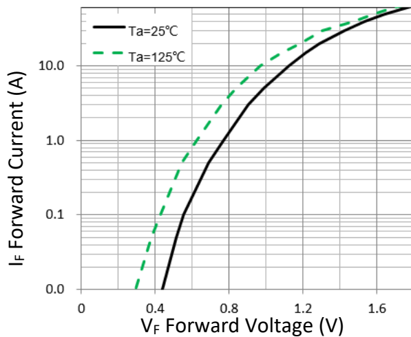
Figure 1. Forward Characteristic(typ.)
