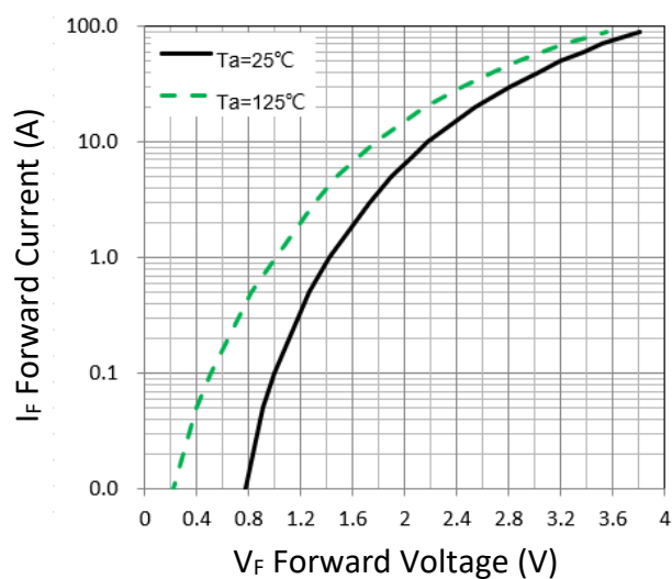
Figure 1. Forward Characteristic(typ.)
