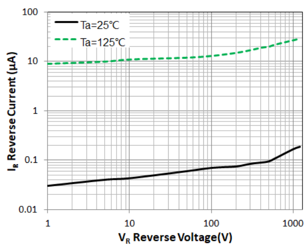
Figure 2. Reverse Characteristic(typ.)
