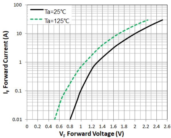
Figure 1. Forward Characteristic(typ.)
