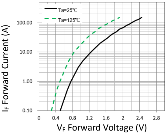
Figure 1. Forward Characteristic(typ.)
