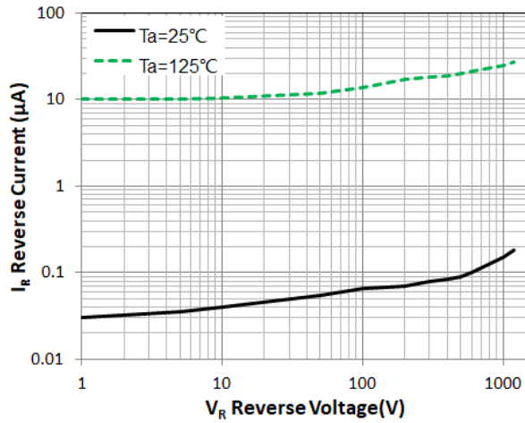
Figure 2. Reverse Characteristic(typ.)
