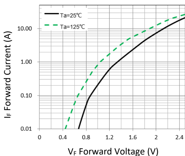
Figure 1. Forward Characteristic(typ.)
