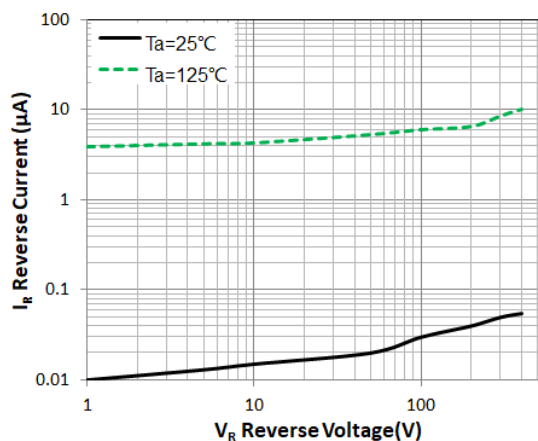
Figure 2. Reverse Characteristic(typ.)
