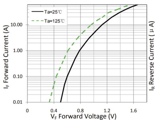
Figure 1. Forward Characteristic(typ.)
