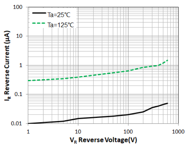
Figure 2. Reverse Characteristic(typ.)
