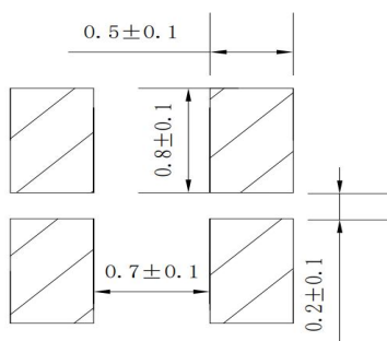
Recommended Solder Pad Design 推荐焊盘设计
