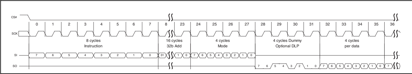
Figure 88 DDR Fast Read initial access (4-byte address, 0Eh or 0Dh [ExtAdd = 1], EHPLC = 01b) [53]
