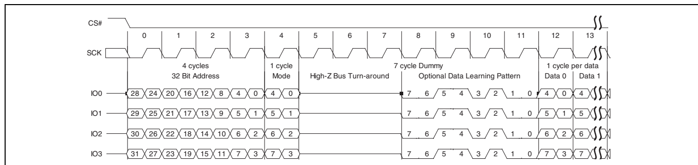
Figure 97 Continuous DDR Quad I/O Read subsequent access (4-byte address, EHPLC = 01b) [55]
