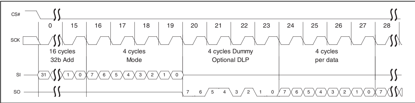
Figure 89 Continuous DDR Fast Read subsequent access (4-byte address [ExtAdd = 1], EHPLC = 01b) [53]
