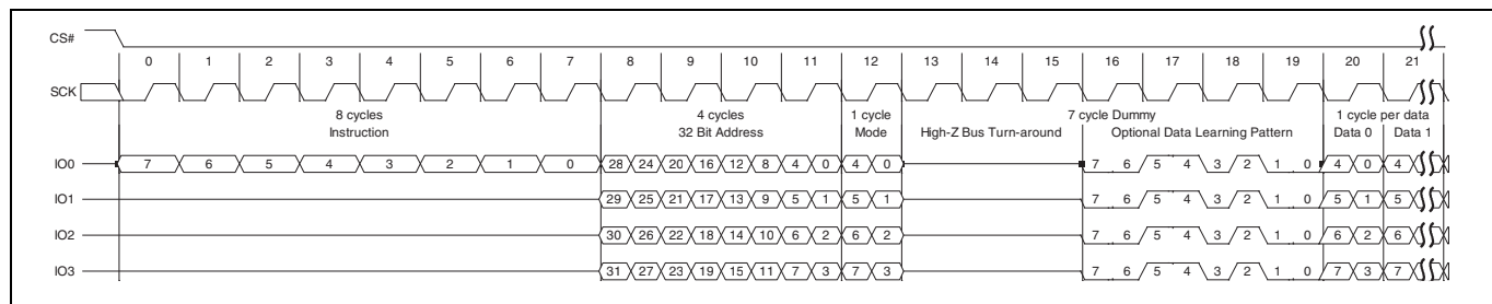
Figure 96 DDR Quad I/O Read initial access (4-byte address, EEh or EDh [ExtAdd = 1], EHPLC = 01b) [54]
