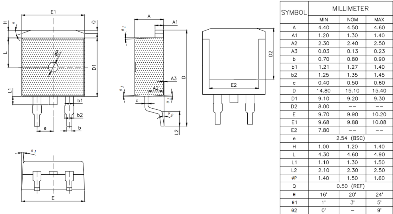
Figure 4. TO-263
