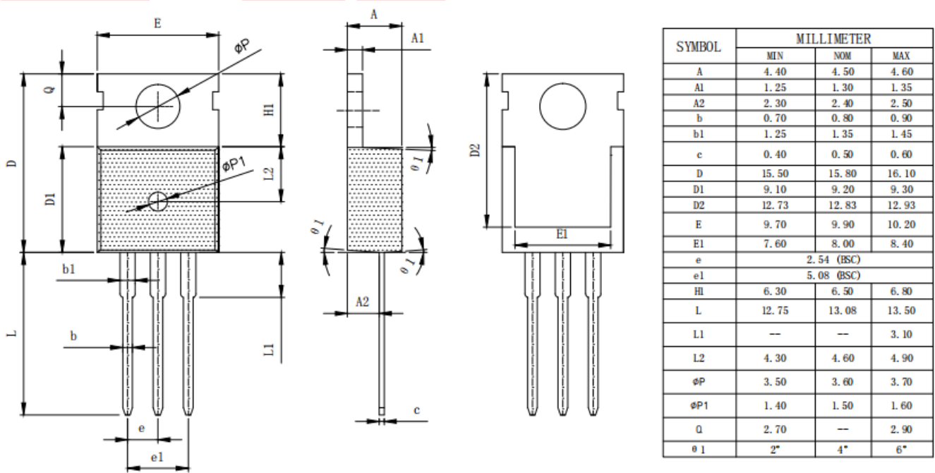
Figure 5. TO-220-FB
