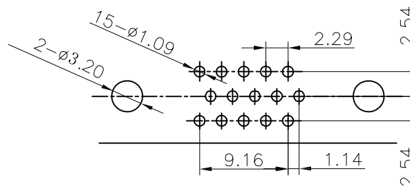
PCB Holes Diagram(Top View)
