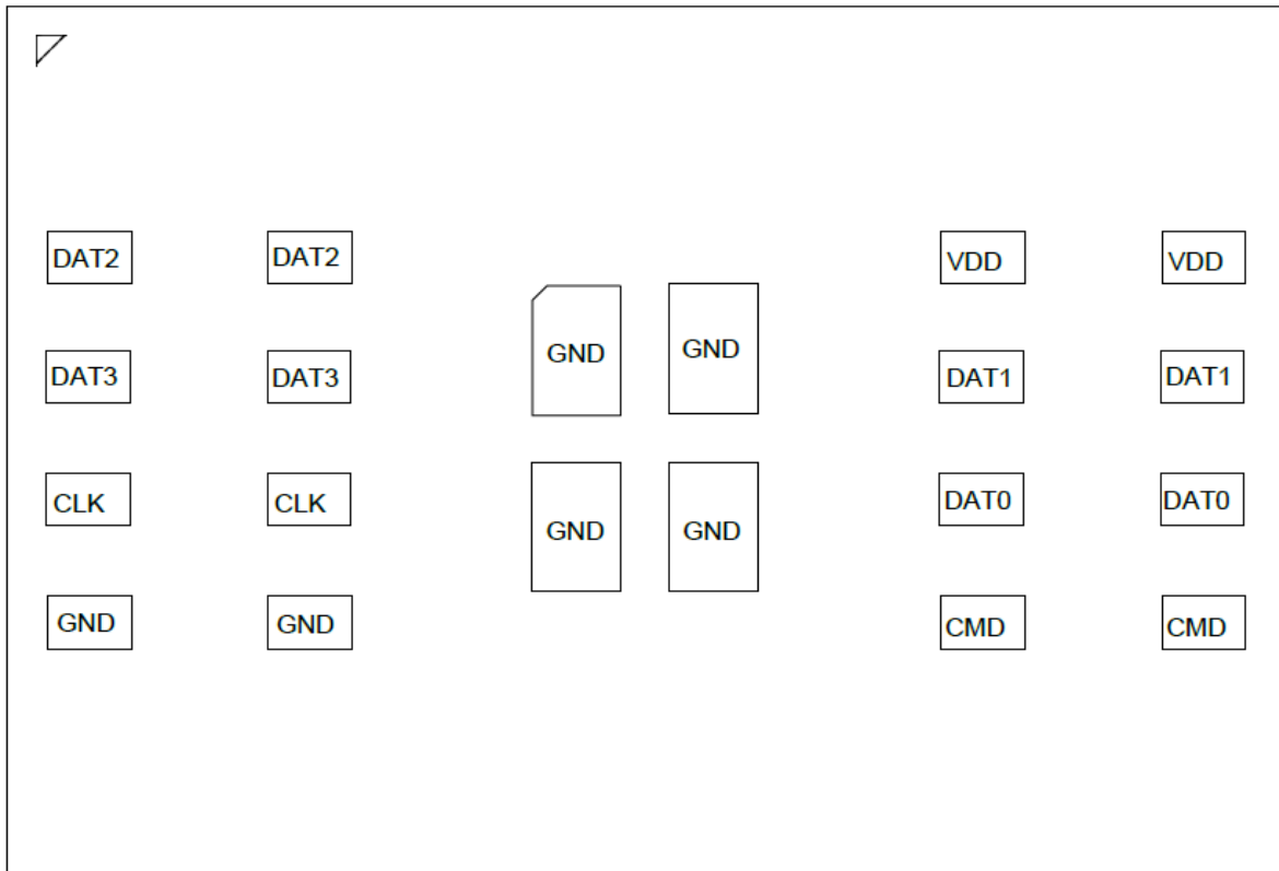
Top view through package
