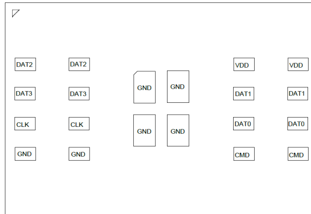
TOP VIEW Through the pckag
