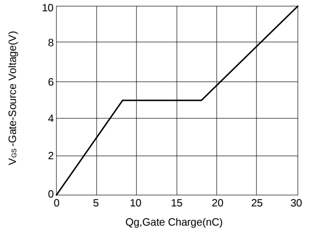
Figure 8: Gate Charge vs Gate to Source Voltage
