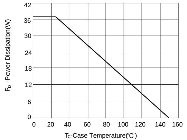
Figure 10: Power Dissipation vs Case Temperature
