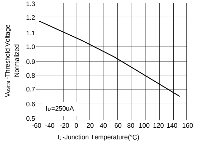
Figure 4: Threshold Voltage vs Junction Temperature
