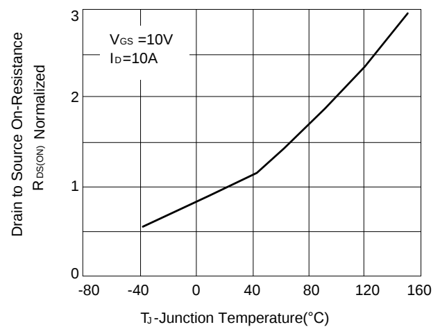
Figure 6: Drain to Source On-Resistance vs Junction Temperature
