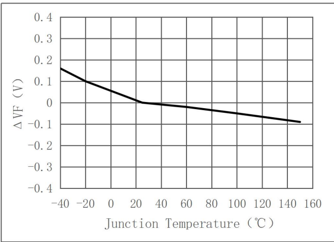
Relative Forward Voltage vs. Junction Temperature ( Δ VF=VF-VF(25℃)=f(Tj) @IF=140mA )
