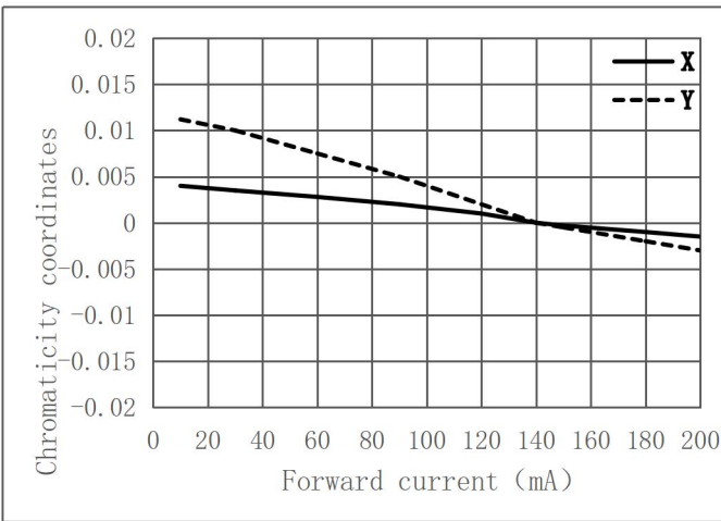
Chromaticity Coordinate Shift ( Δ CIE x, Δ CIE y=f(IF) @ Ts =25℃ )
