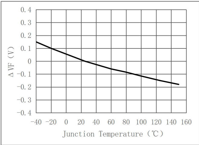
Relative Forward Voltage vs. Junction Temperature ( \Delta VF = VF - VF(25^\circ C) = f(T_j) @ I_F = 140\text{mA} )
