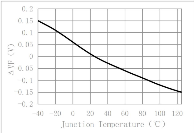
Relative Forward Voltage (Green ΔVF)
