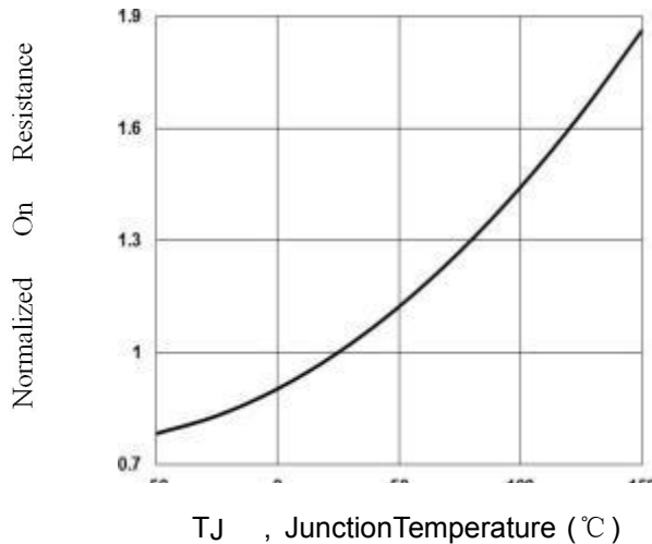
Fig. 3 Normalized R_{DS(on)} vs. T_J
