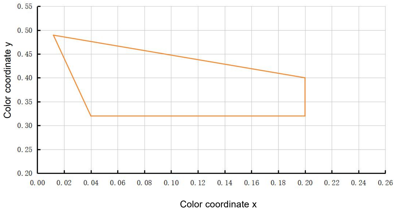
Bin Range of Chromaticity Coordinates Specifications
