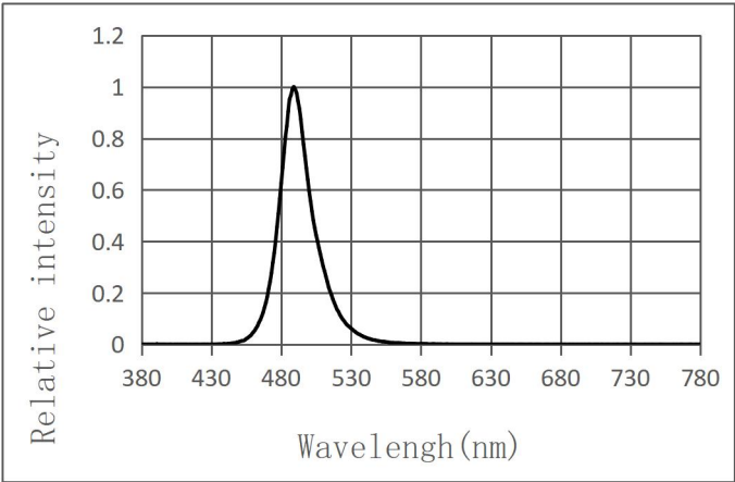
Spectrum Distribution (@IF = 200 mA; T=25℃ )
