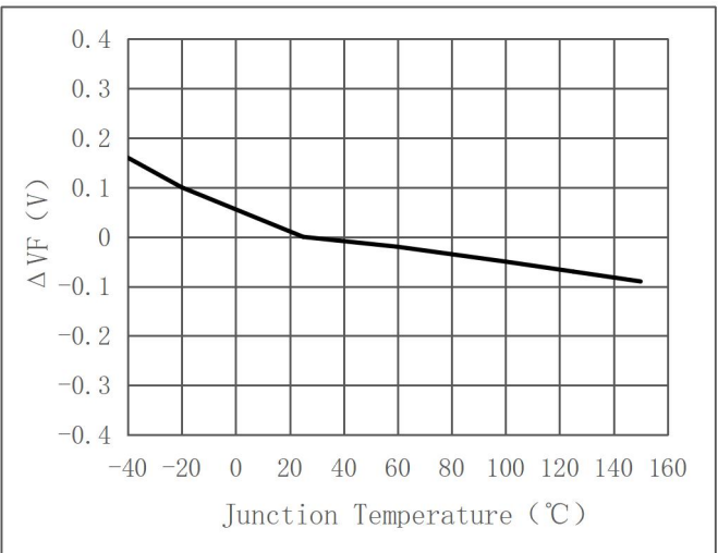
Relative Forward Voltage vs. Junction Temperature ( \Delta VF=VF-VF(25^\circ C)=f(T_j) @IF=200mA )
