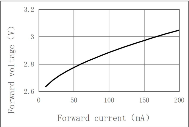
Forward current VS. Forward voltage (@T = 25℃)
