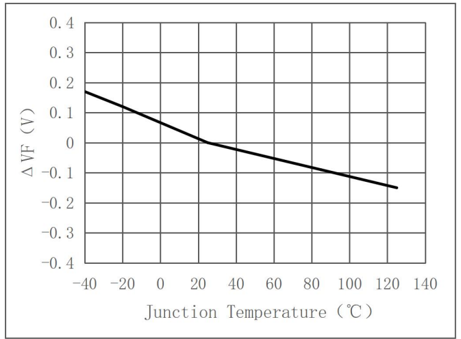
Relative Forward Voltage vs. Junction Temperature (△ VF=VF-VF(25° C)=f(Tj) @IF=50mA)
