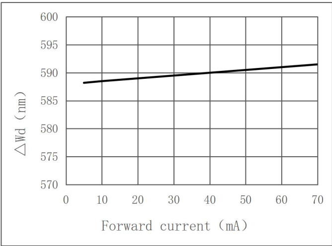
Wavelength Vs. forward Current (△ Wd =Ts = 25° C)
