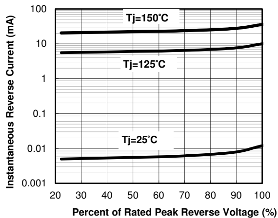
FIG.3-TYPICAL REVERSE CHARACTERISTICS
