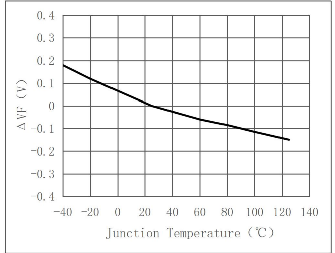
Relative Forward Voltage vs. Junction Temperature ( \Delta VF=VF-VF(25℃)=f(Tj) @IF=140mA )
