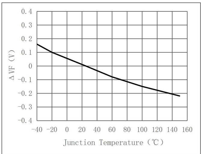
Relative Forward Voltage vs. Junction Temperature ( \Delta V_F = V_F - V_F(25^\circ \text{C}) = f(T_j) @IF=200mA)
