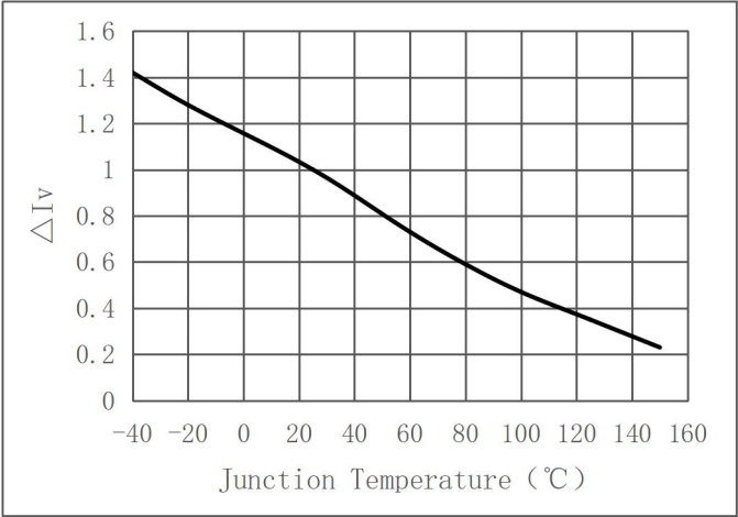
Relative Luminous Intensity vs. Junction Temperature ( \Delta I_v = I_v / I_v(25^\circ \text{C}) = f(T_j) IF=200mA)
