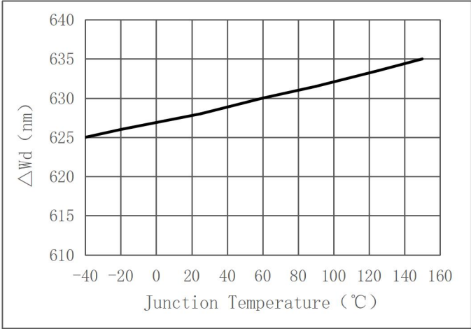
Dominant wavelength shift vs. Junction Temperature ( \lambda_{\text{dom}} = f(T_j) ; IF = 200mA)
