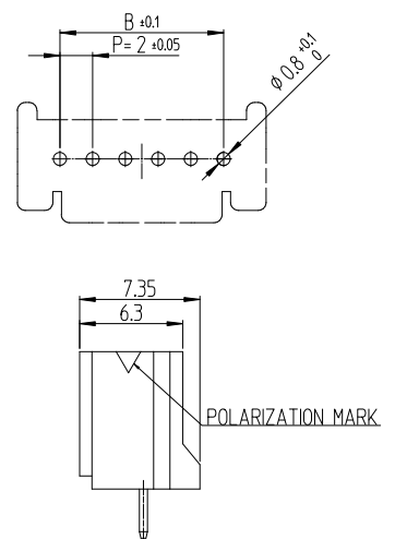
Recommended PCB Layout (t=1.6mm)
