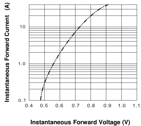
FIG.4-TYPICAL FORWARD CHARACTERISTICS
