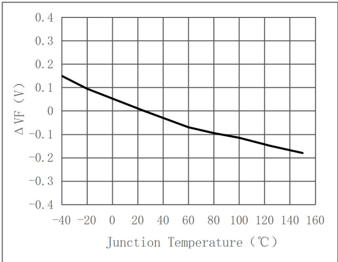
Relative Forward Voltage vs. Junction Temperature ( \Delta VF = VF - VF(25^\circ C) = f(T_j) @ I_F = 200\text{mA} )
