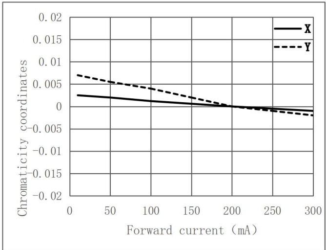
Chromaticity Coordinate Shift ( \Delta CIE\ x, \Delta CIE\ y = f(I_F) @ T_s = 25^\circ C )
