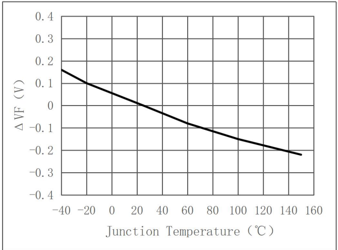
Relative Forward Voltage vs. Junction Temperature ( \Delta V_F = V_F - V_F(25^\circ \text{C}) = f(T_j) @IF=140mA)
