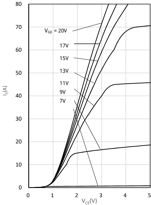
Fig. 5 Output characteristics
