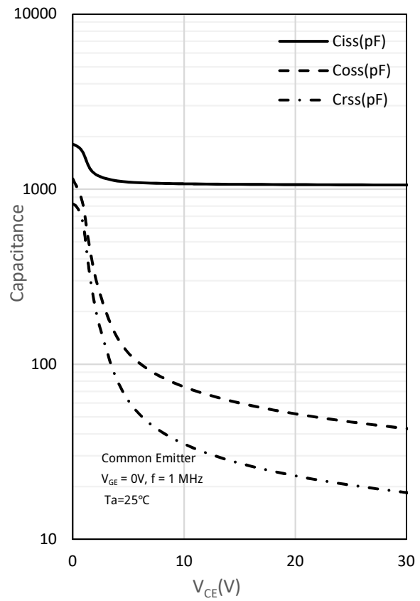
Fig. 12 Capacitance characteristics
