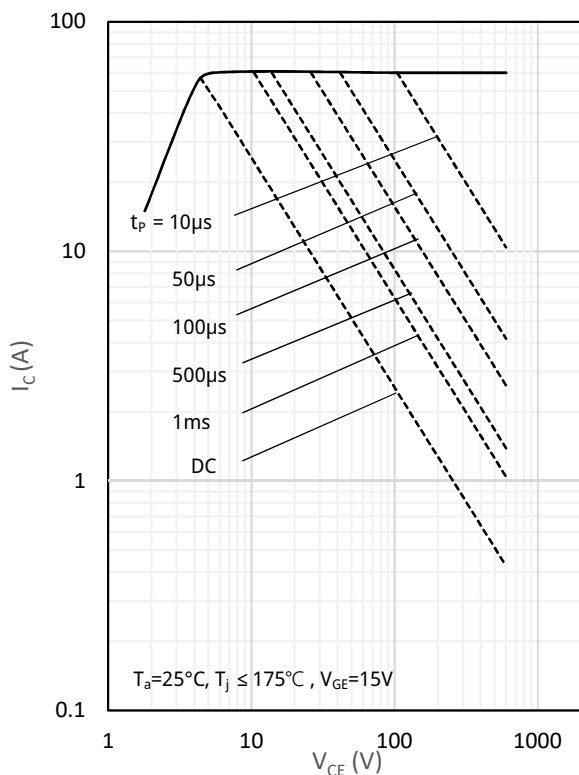
Fig. 1 FBSOA characteristics for TO-220F
