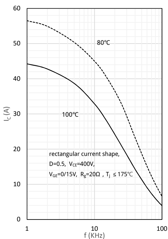
Fig.4 Load Current vs. Frequency TO-220 and TO-263
