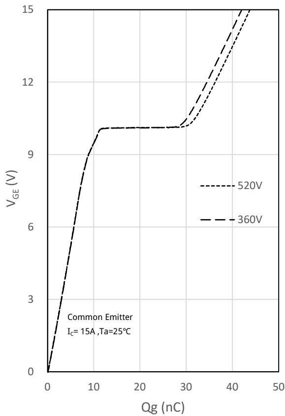
Fig. 11 Gate charge characteristics
