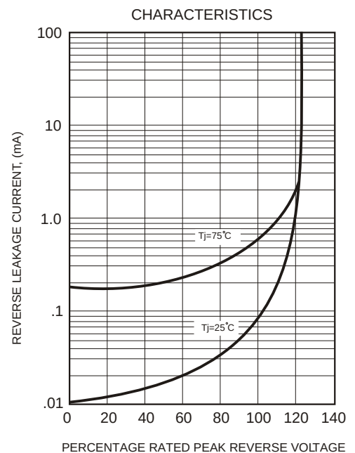
FIG.5 - TYPICAL REVERSE
