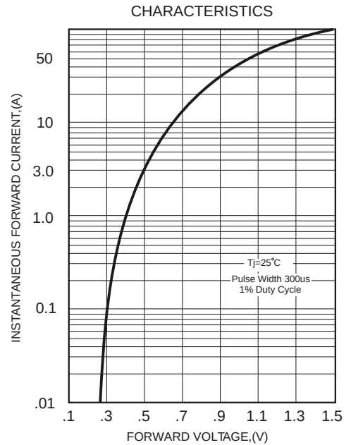
FIG.2-TYPICAL FORWARD
