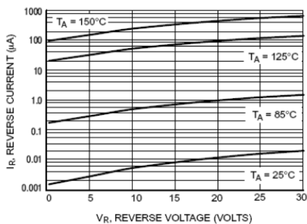
Figure 2. Leakage Current
