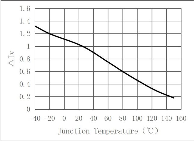
Relative Luminous Intensity vs. Junction Temperature ( \Delta I_v = I_v / I_v(25^\circ \text{C}) = f(T_j) IF=200mA)
