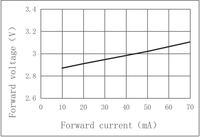
Forward current VS. Forward voltage (@T = 25℃)
