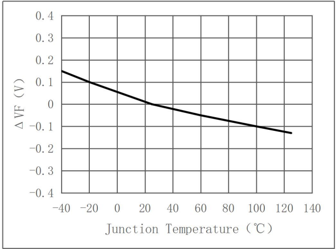
Relative Forward Voltage vs. Junction Temperature ( Δ VF=VF-VF(25℃)=f(Tj) @IF=50mA )
