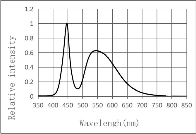
Spectrum Distribution (@IF = 50 mA; T=25℃ )
