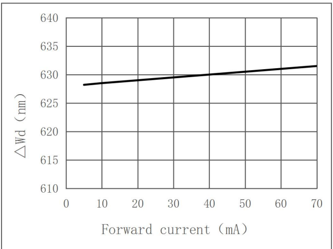
Wavelength Vs. forward Current ( \Delta W_d = T_s = 25^\circ \text{C} )
