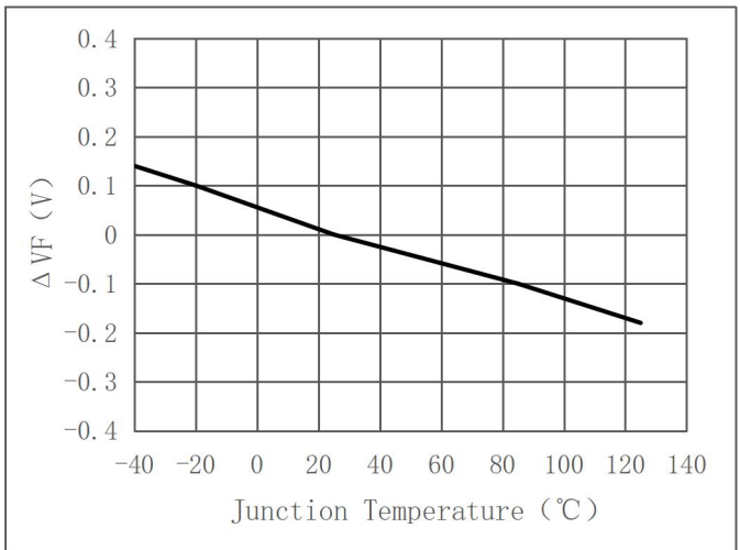
Relative Forward Voltage vs. Junction Temperature ( \Delta V_F = V_F - V_F(25^\circ \text{C}) = f(T_j) @IF=50mA)
